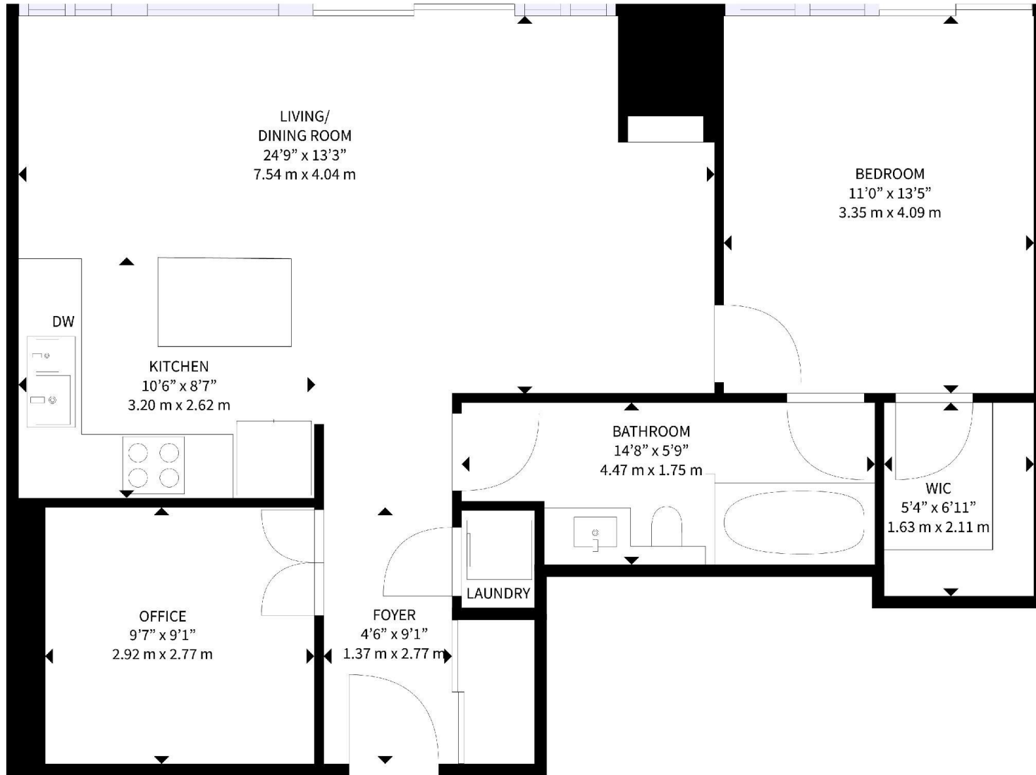
FLOOR PLAN
