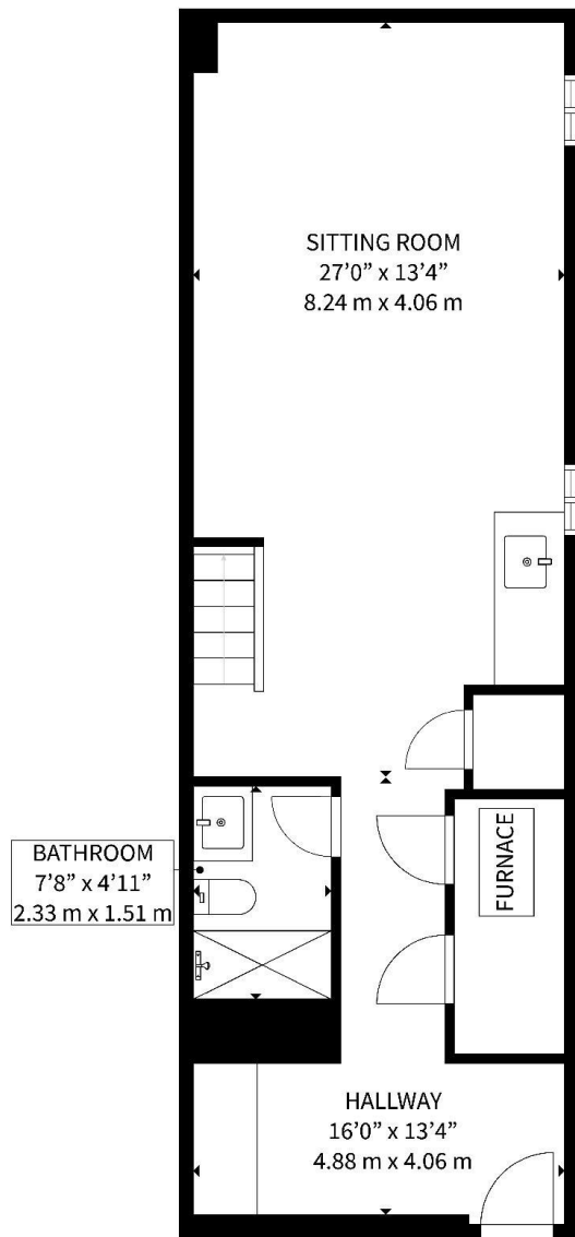
BASEMENT
