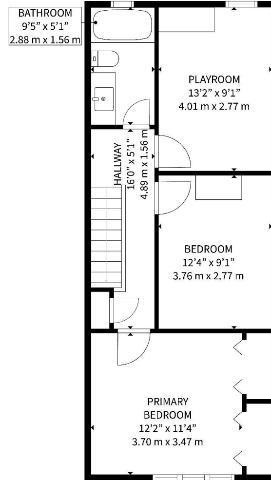
FLOOR 2
